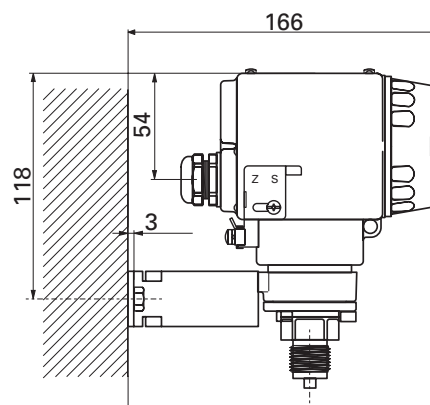
Fig. 7 Wall mounting
