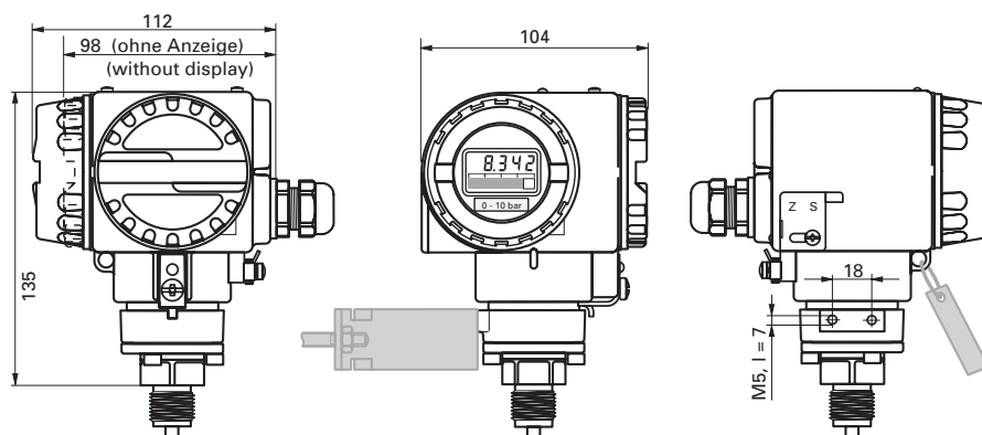
Fig. 1 Dimensions [mm]
