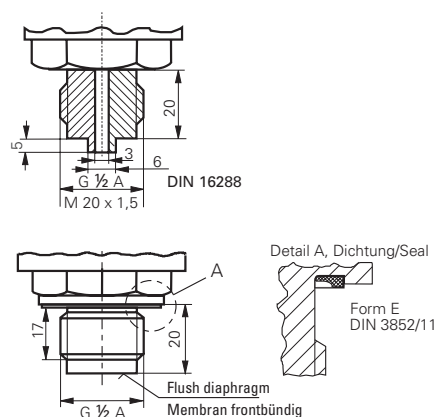
Fig. 5 Process couplings for Polisilicone sensor
