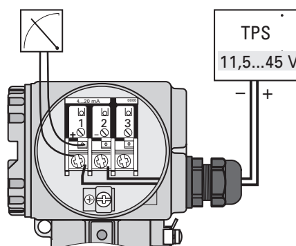
Fig. 3 Electrical connections
