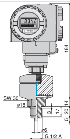
Fig. 2 Temperature isolator
