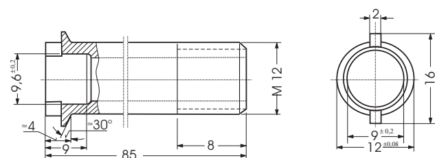
fig. 4 threaded fitting 85mm
