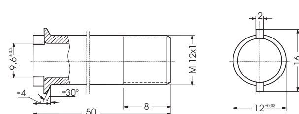
fig. 7 threaded fitting 50 mm
