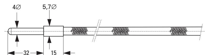
fig. 2 Pencil-type thermocouple D
