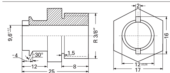
fig. 6 threaded fitting 25 mm
