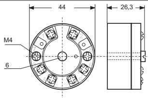
Fig 2 Connection resistance thermometer
