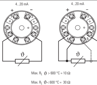
Fig 3 Connection thermocouple
