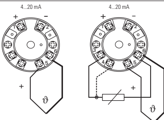
Fig 4 Connection potentiometer
